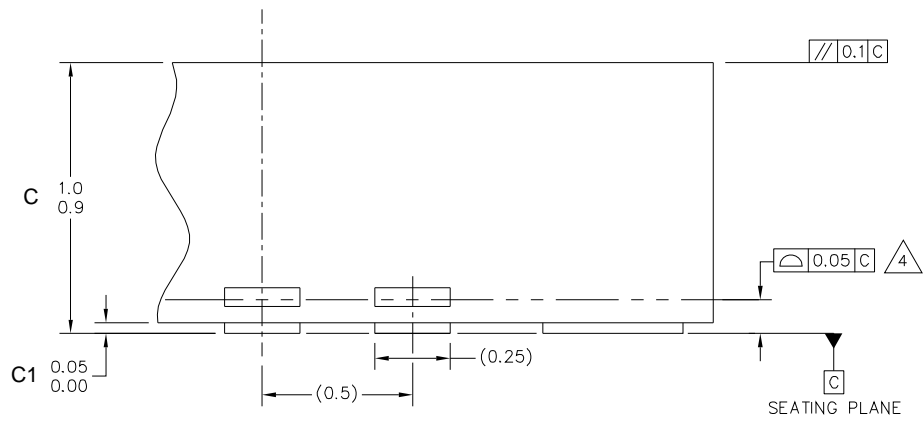
DETAIL G
