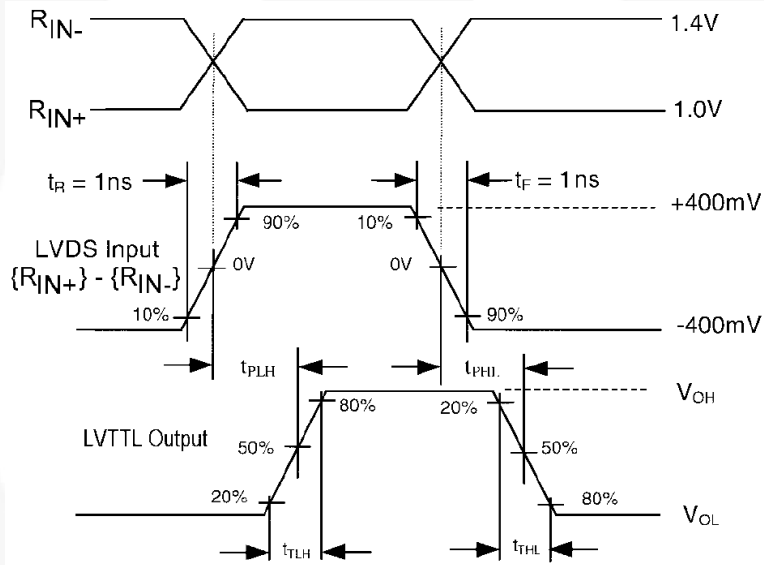
Figure 4. LVDS Input to LVTTTL Output AC Waveforms
