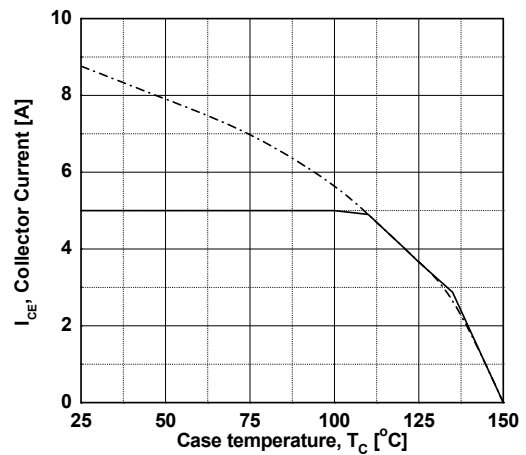
Figure 18. Current Derating
