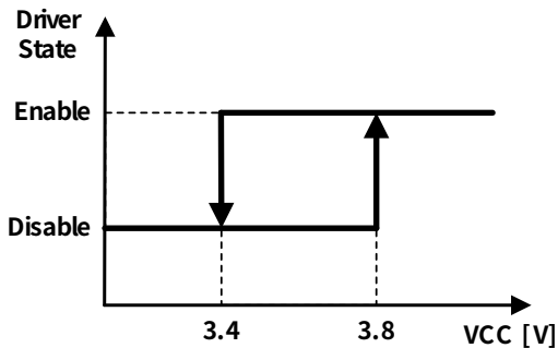
Figure 28. UVLO on VCC
