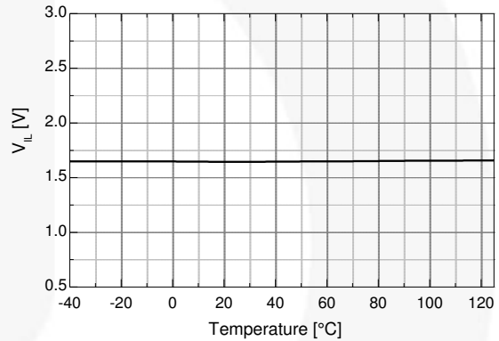
Figure 25. Logic LOW Input Voltage vs. Temperature
