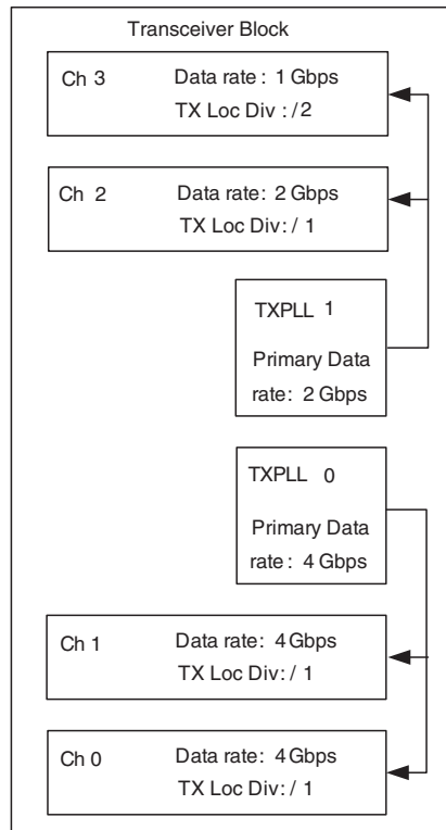
Figure 2-109. Resultant Transceiver Block Configuration with Two TXPLLs
