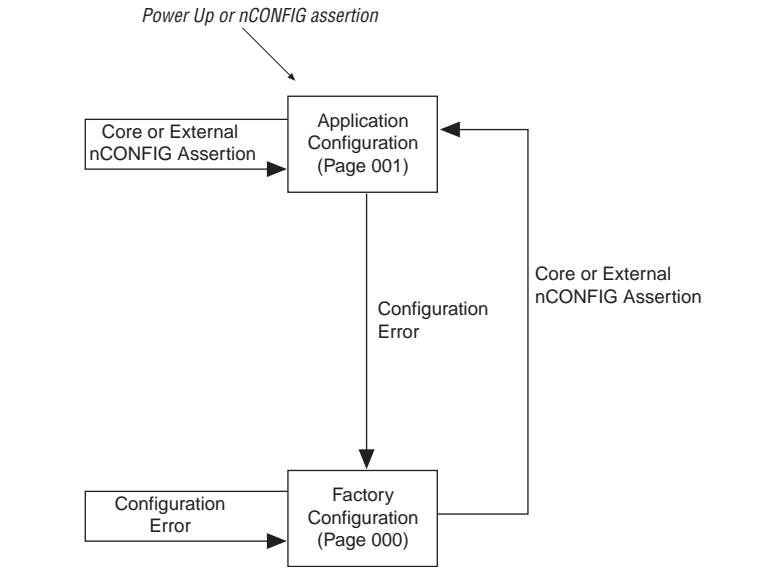
Figure 14–5. Transitions Between Configurations in Local Update Mode
