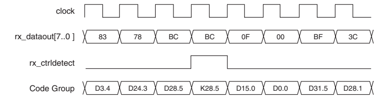
Figure 2–84. Control Code Detection
