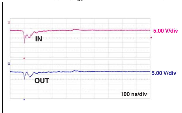
Figure 9. ESD response to IEC 61000-4-2 (-15 kV air discharge) on one EAR input ( V_{in} ) and on one EAR output
