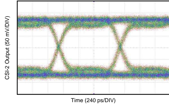
Figure 41. CSI-2 Data Output at 1040 Mbps
