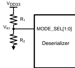
Figure 28. MODE_SEL[1:0] Connection Diagram
