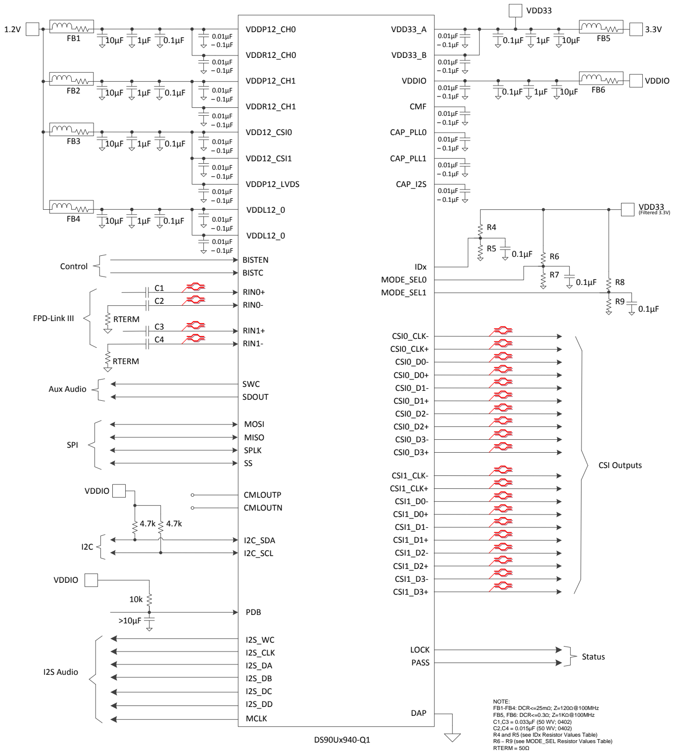
Figure 37. Typical Connection Diagram (Coax)
