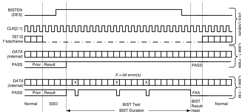
BIST Waveforms
