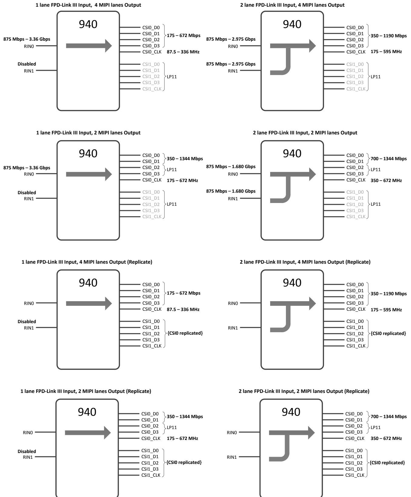
Figure 27. Datapath Configurations
