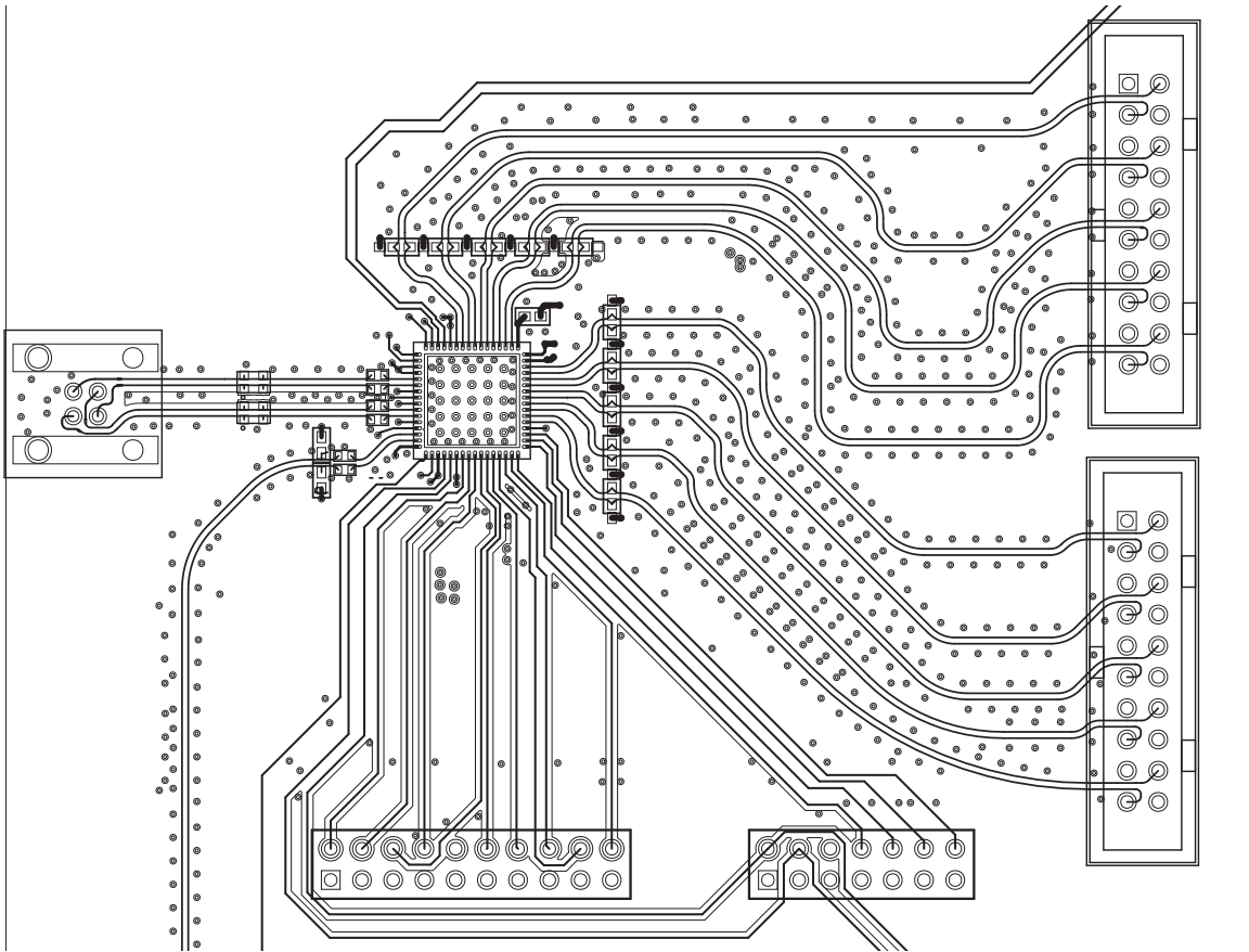
Figure 43. DS90UB940-Q1 Deserializer Example Layout
