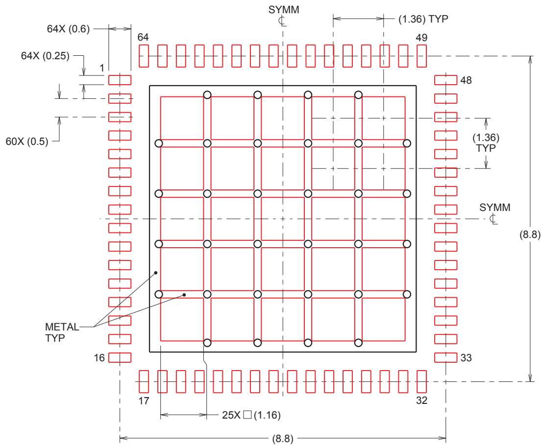
Figure 42. 64-Pin WQFN Stencil Example of Via and Opening Placement (dimensions in mm)
