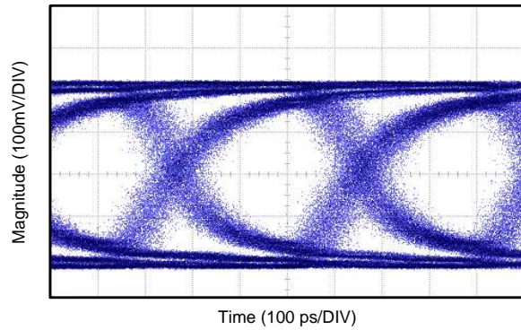
Figure 40. Loop-through CML Output at 2.6 Gbps Serial Line Rate
