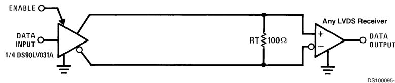
FIGURE 6. Point-to-Point Application
