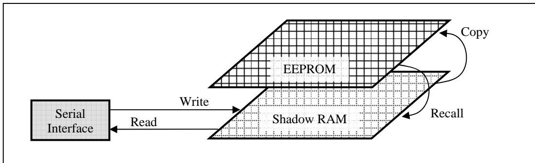
Figure 21. EEPROM Access via Shadow RAM
