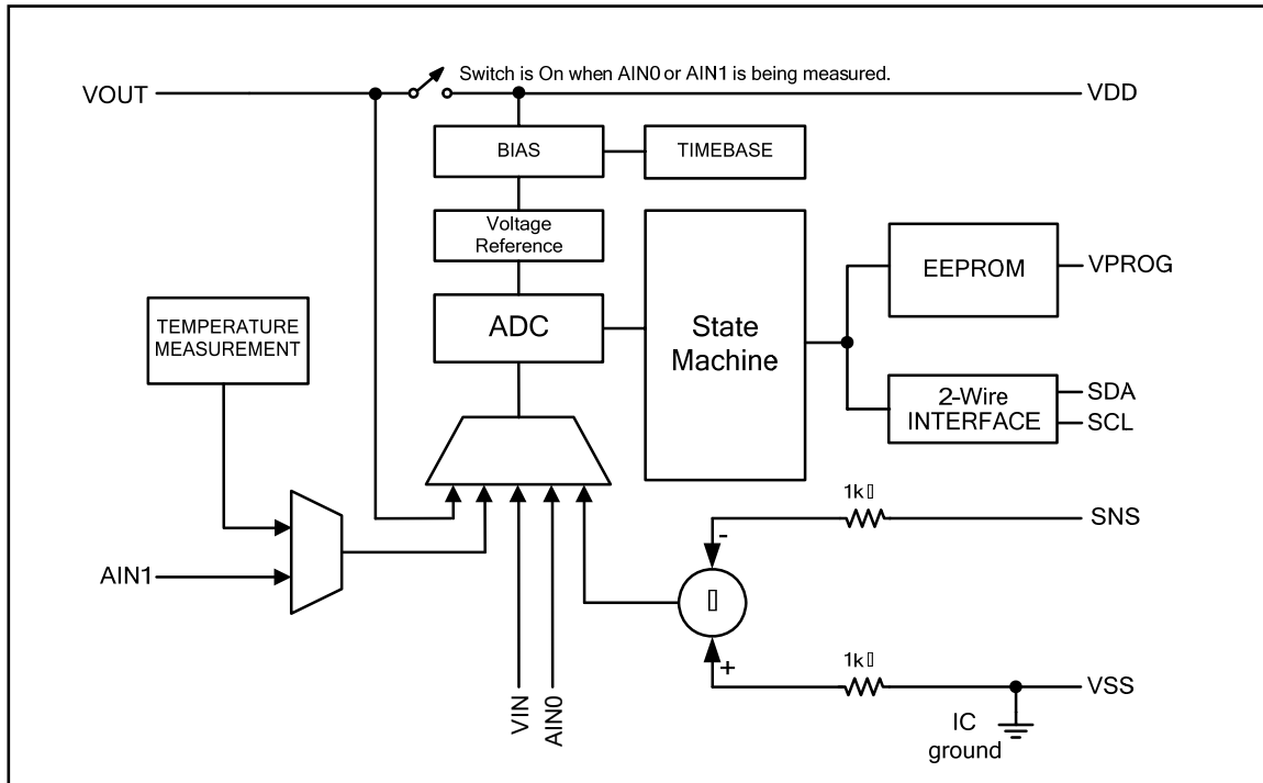
Figure 2. Block Diagram
