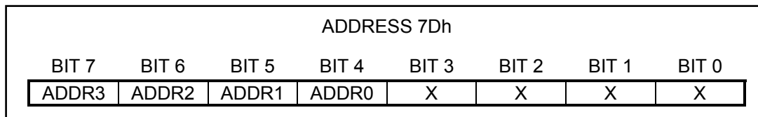
Figure 24. I 2 C Address Register Format
