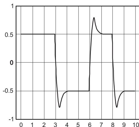
Figure 2. Idealized De-Emphasis Waveform
