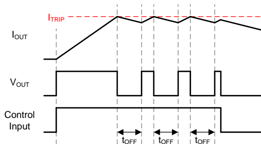
Figure 4. Off-Time Current-Regulation
