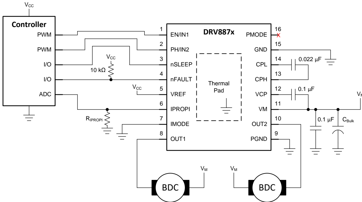
Figure 15. Typical Application Schematic
