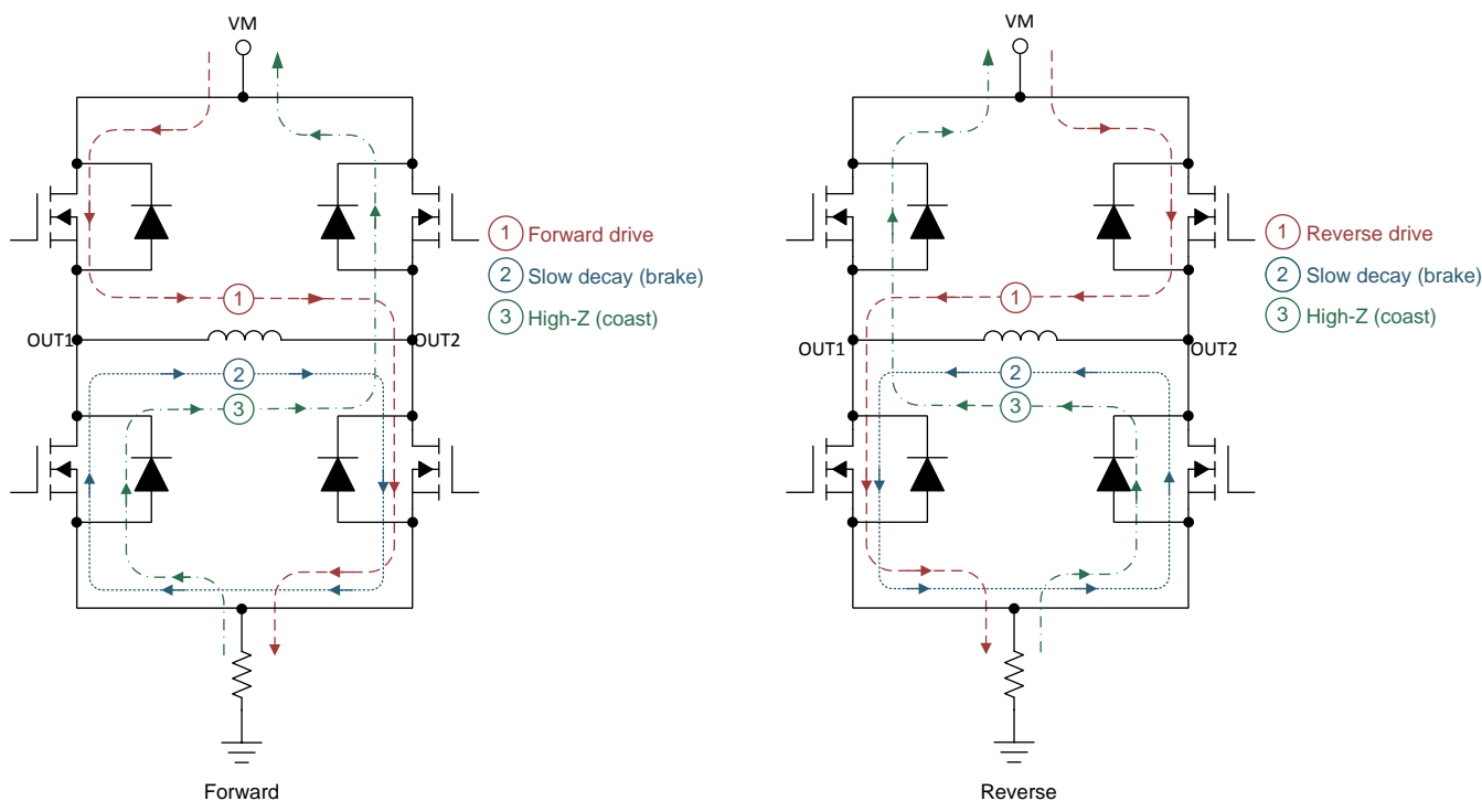
Figure 2. H-Bridge States
