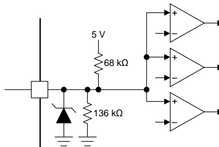
Figure 9. Quad-Level Input
