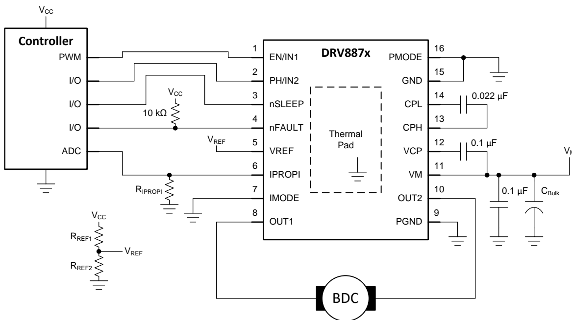
Figure 10. Typical Application Schematic
