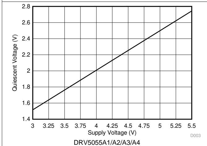
Figure 3. Quiescent Voltage vs Supply Voltage
