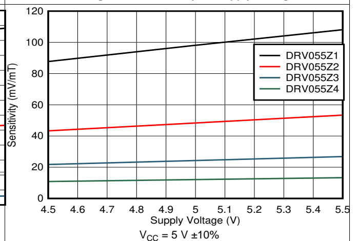
Figure 12. Sensitivity vs Supply Voltage
