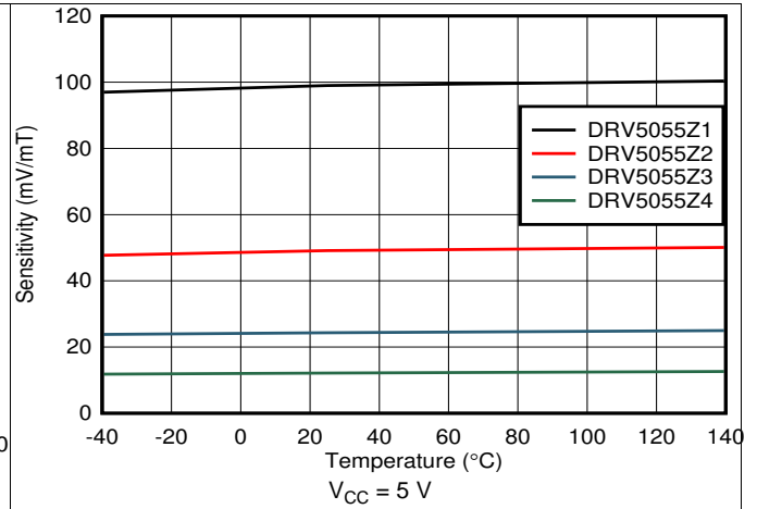
Figure 8. Sensitivity vs Temperature
