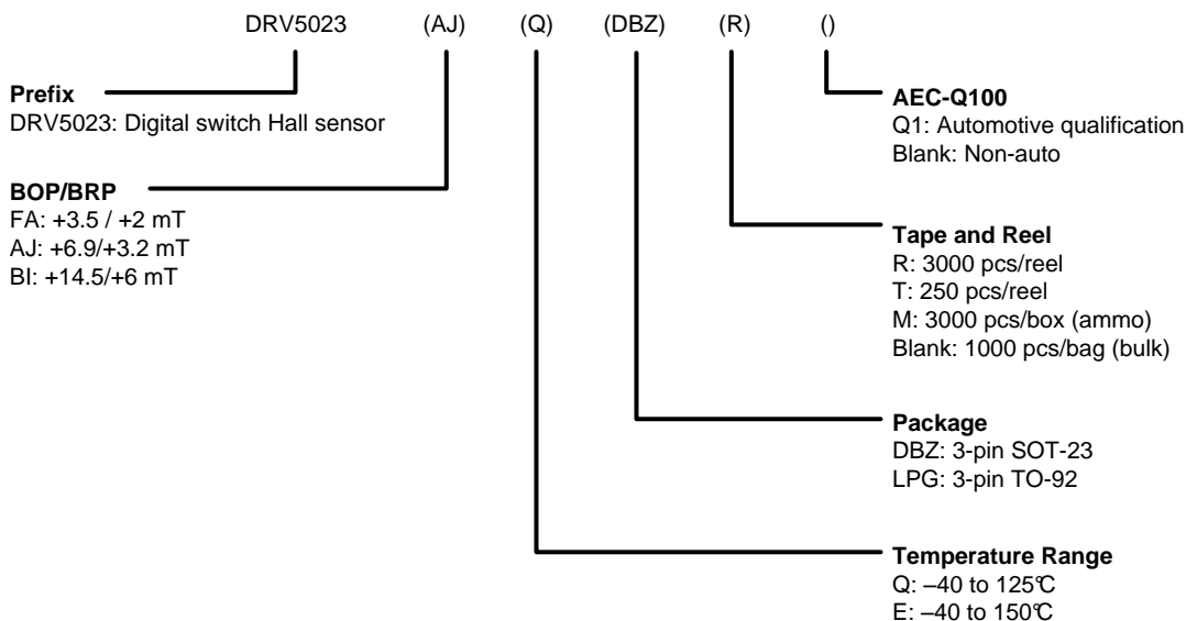
Figure 23. Device Nomenclature
