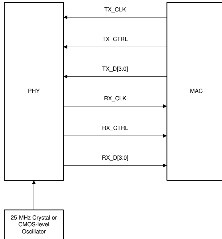
Figure 8-13. RGMI Connections
