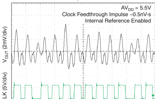
CLOCK FEEDTHROUGH 2MHz, MIDSACLE
