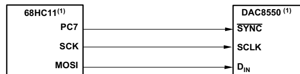
Figure 54. DAC8550 to 68HC11 Interface
