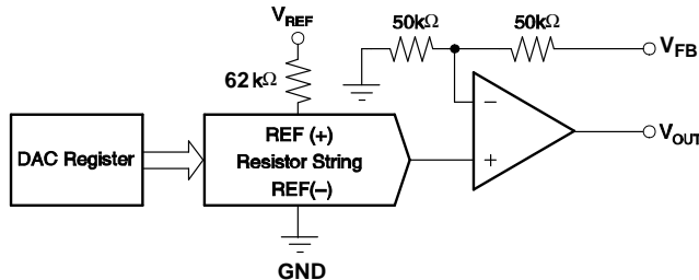
Figure 47. DAC8550 Architecture
