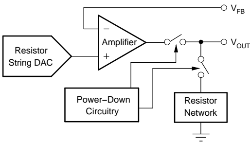
Figure 51. Output Stage During Power-Down
