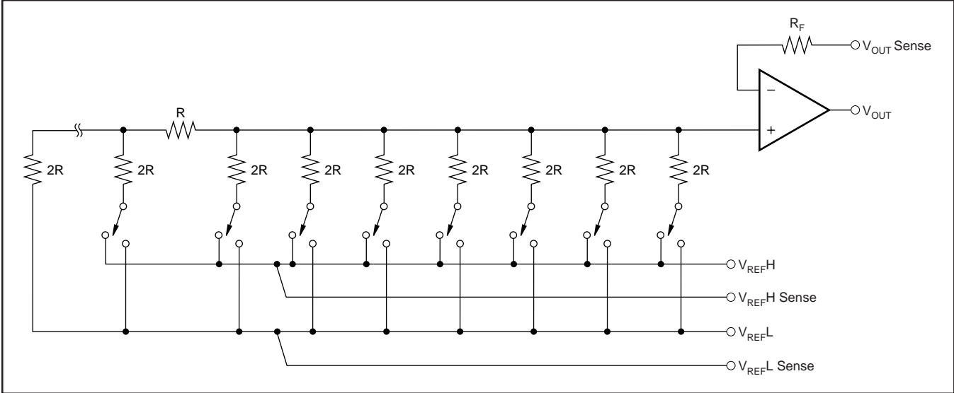
FIGURE 1. DAC7644 Architecture.
