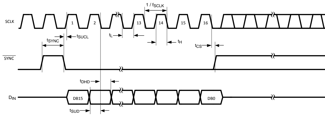
Figure 2. DAC121S101 Timing
