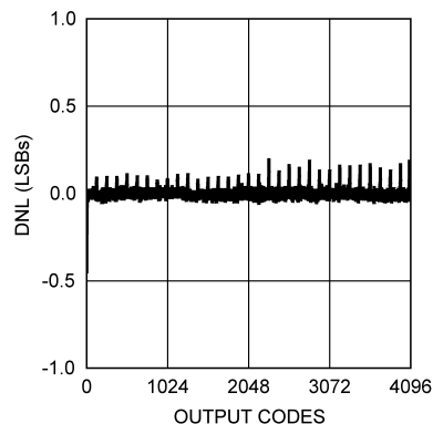
DNL vs. Output Code
