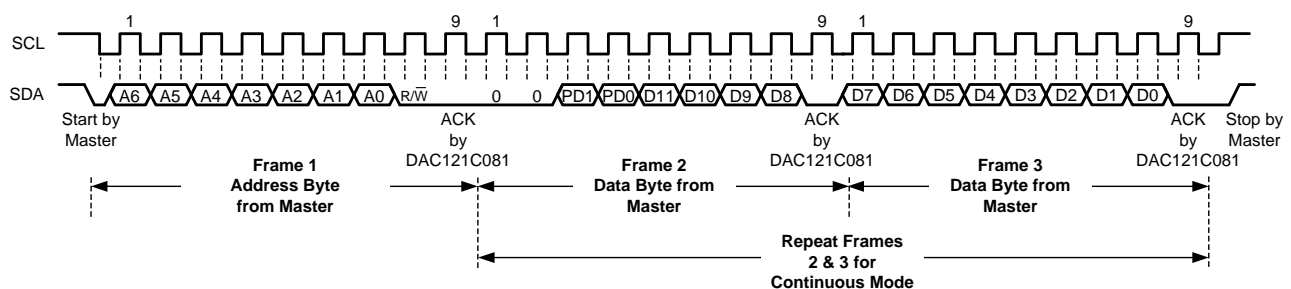
Figure 23. Typical Write to the DAC Register
