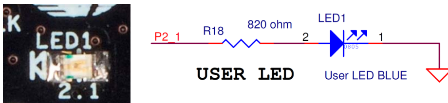
Figure 4-13. User LED
