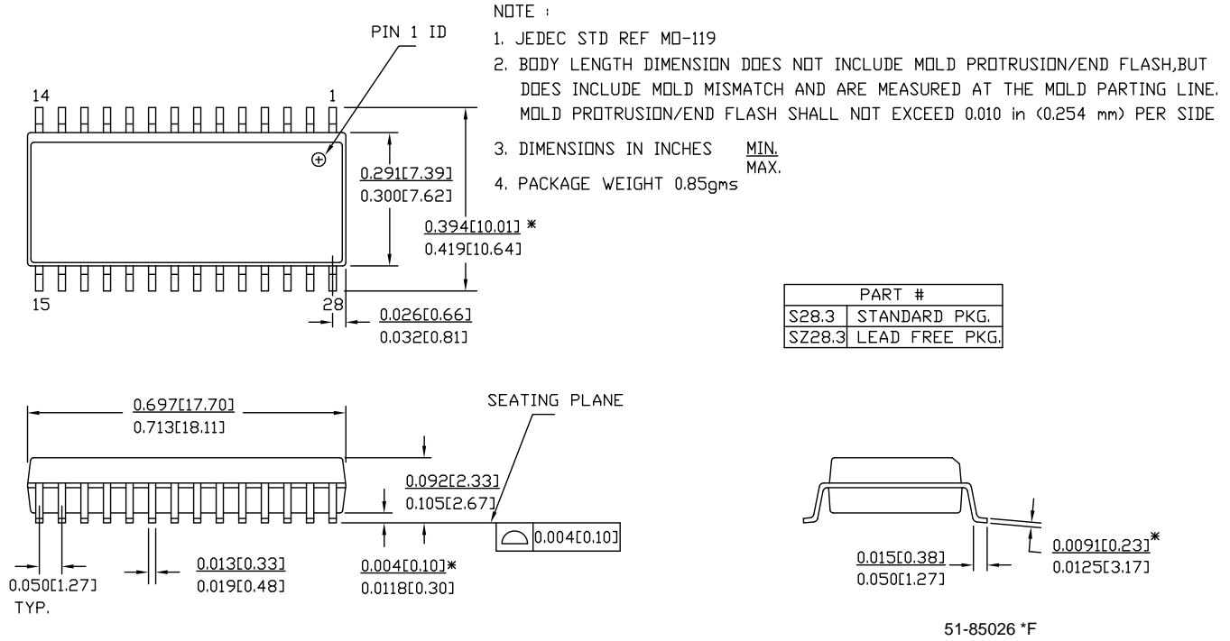
Figure 8. 28-pin SOIC
