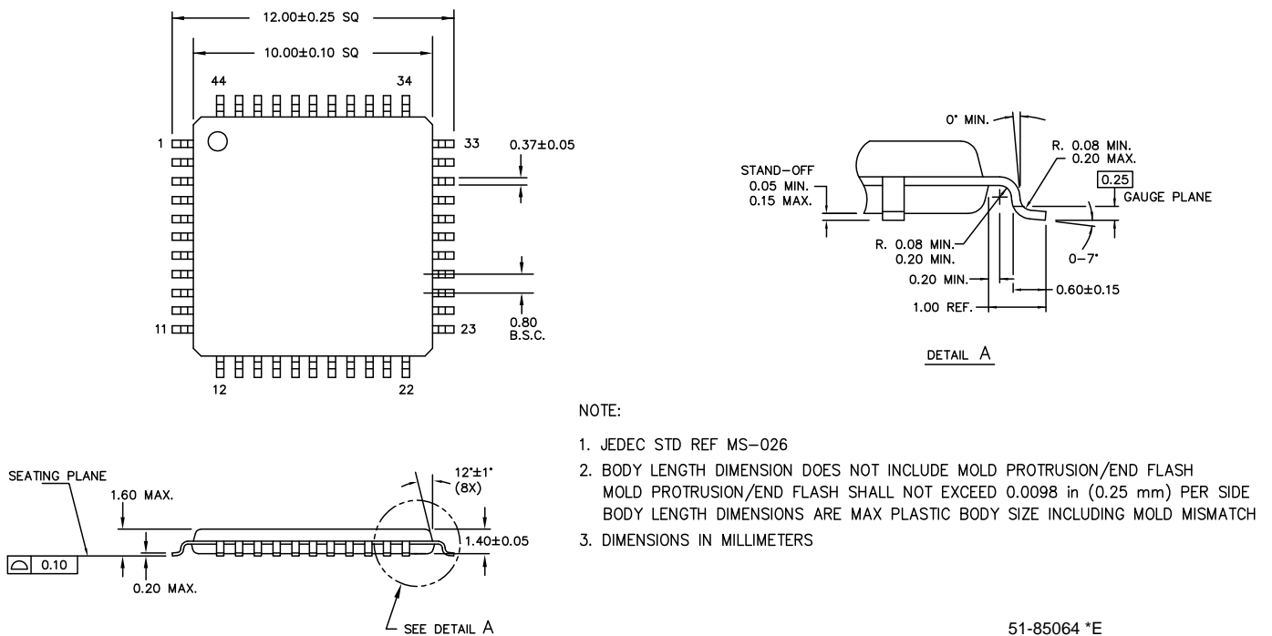
Figure 9. 44-pin TQFP
