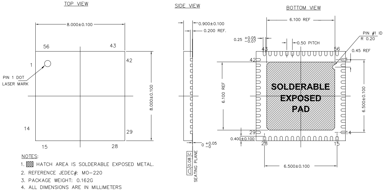
Figure 6. 56-Pin QFN (8 × 8 × 0.90 mm)
