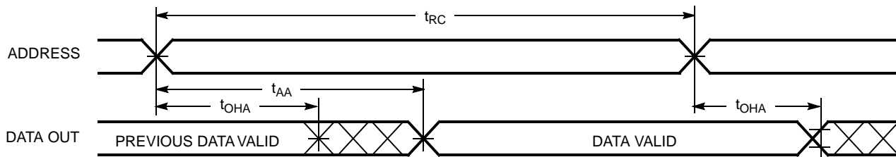
Figure 4. Read Cycle No.2 (Either Port \overline{\text{CE}}/\overline{\text{OE}} Access) [18, 21, 22]
