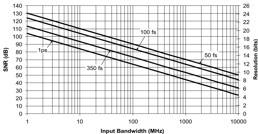
Figure 35. Data Converter Jitter Requirements
