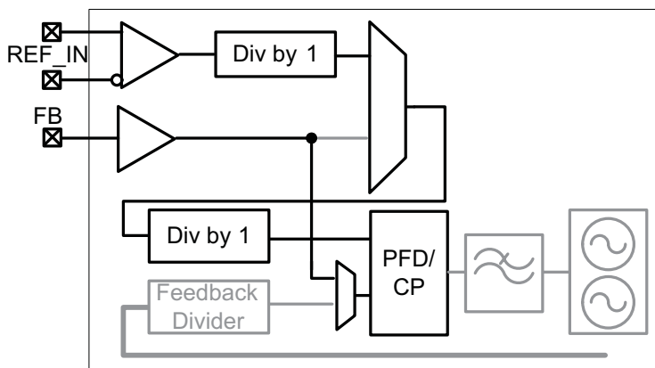
Figure 25. CDCE62002 in External Feedback Mode
