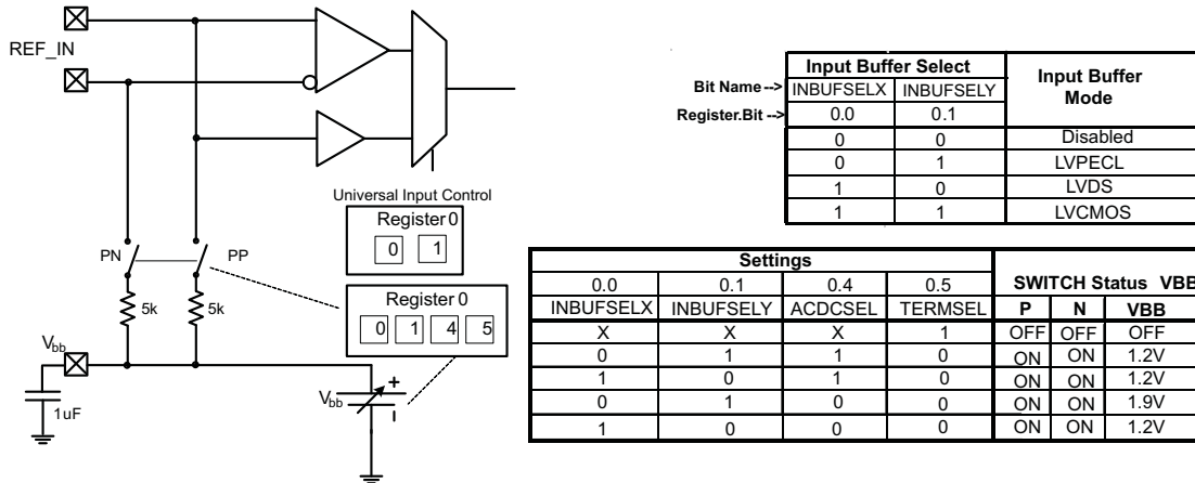
Figure 22. CDCE62002 Universal Input Buffer
