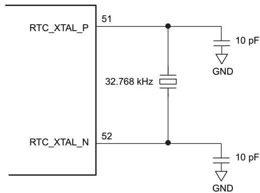
Figure 5-9. RTC Crystal Connections
