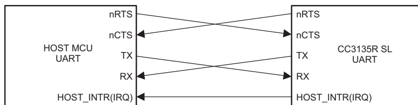
Figure 5-18. 5-Wire UART Topology
