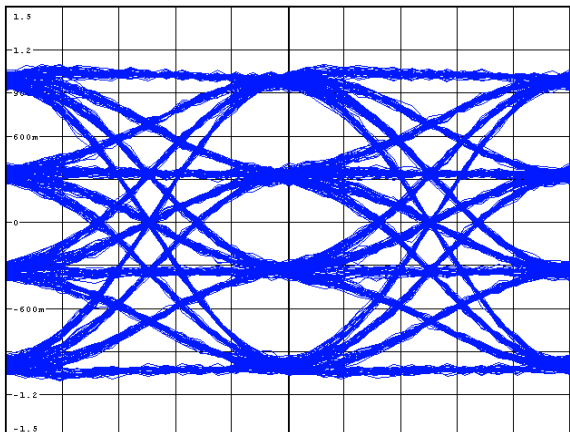
Eye Diagram 1 Mbps 4-GFSK, 400 kHz deviation 500 kHz loop bandwidth
