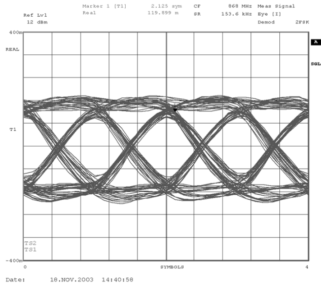
Figure 5-19. GFSK Eye Diagram. 153.6 kBaud, NRZ, ±79.2 kHz Frequency Deviation.
