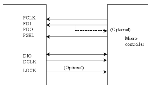
Figure 5-3. Microcontroller Interface
