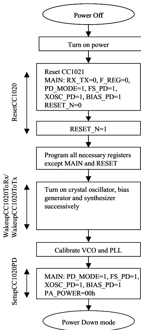
Figure 5-27. Initializing Sequence
