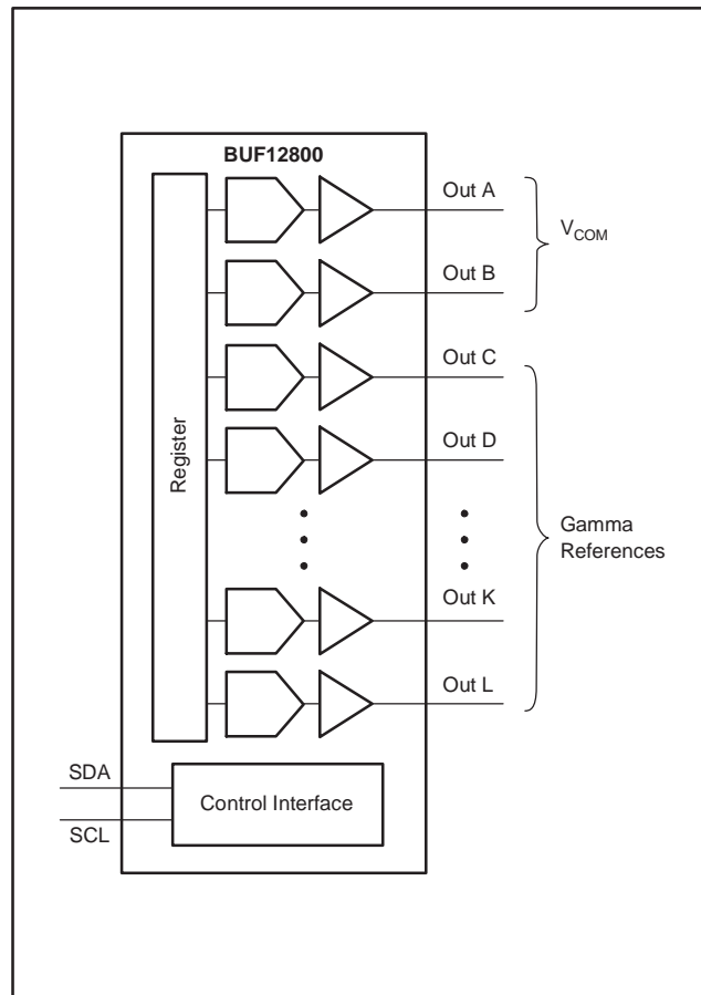
Figure 14. BUF12800 Used for Programmable V_{COM}
