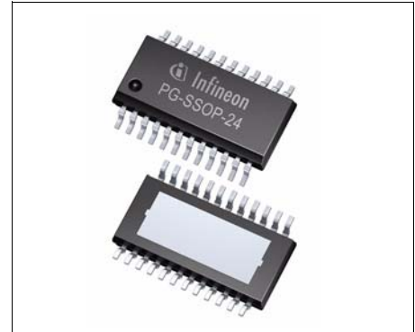
PG-SSOP-24-14 EP
