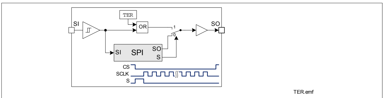
Figure 22 Combinatorial Logic for TER Flag
