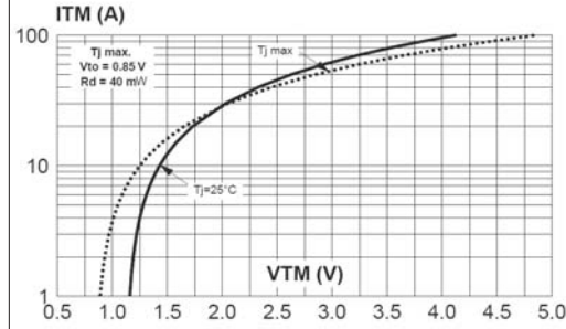
Fig. 4: On-state characteristics (maximum values).
