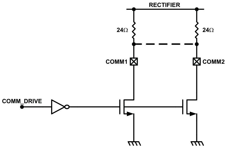
Figure 35. Resistive Load Modulation
