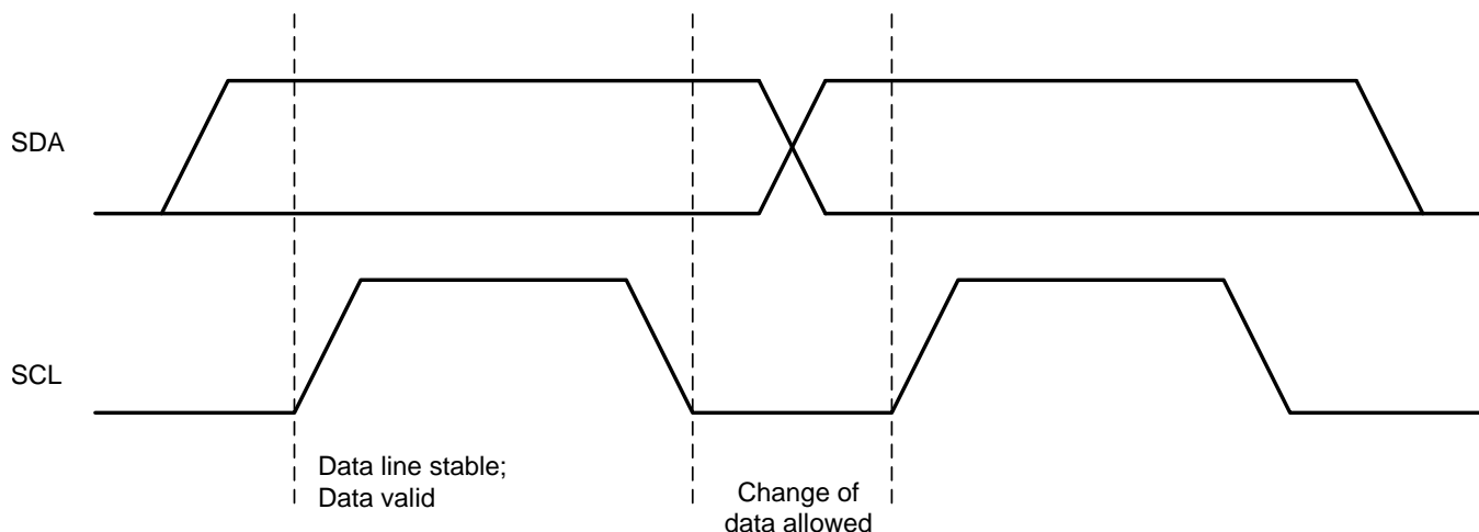
Figure 18. Bit Transfers on the I2C bus
