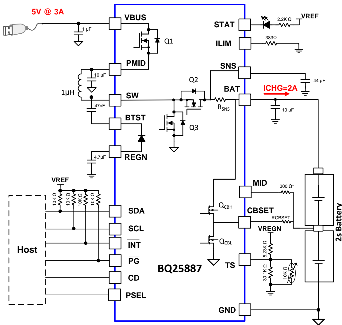
Figure 73. BQ25887 (Cell Balancing and I2C) Typical Application Diagram
