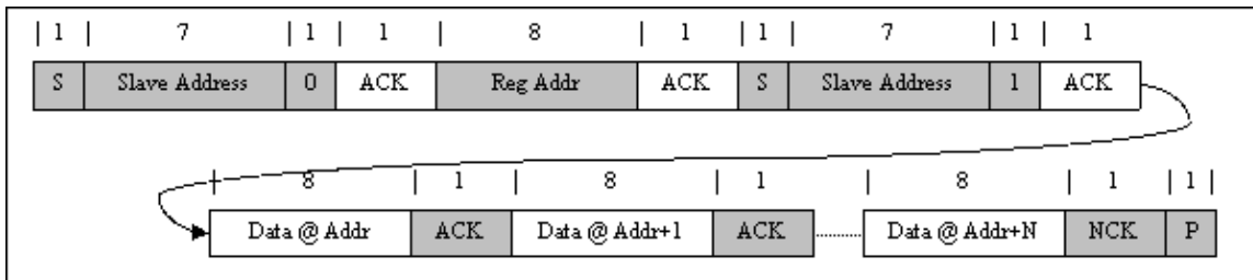
Figure 26. Multi-Read
