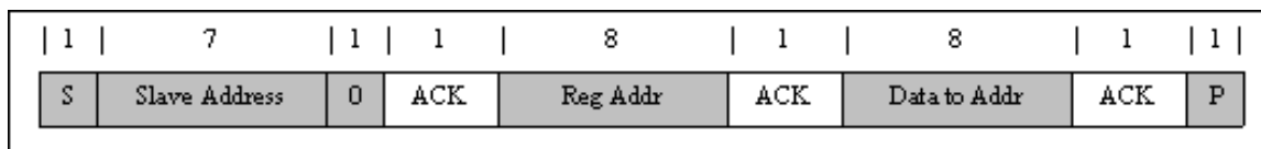
Figure 23. Single Write
