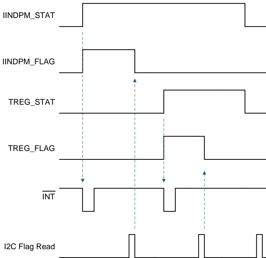
Figure 17. \overline{\text{INT}} Generation Behavior Example
