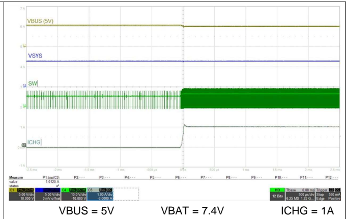
Figure 75. Charge Enable
