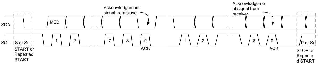
Figure 20. Data Transfer on the I2C Bus
