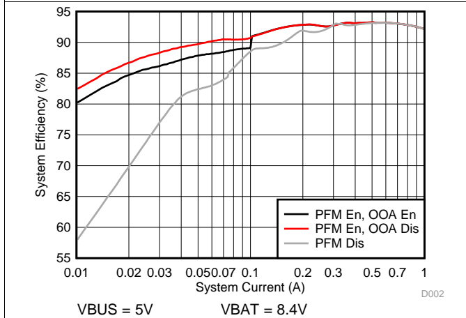
Figure 3. System Efficiency vs. System Current
