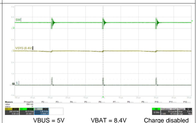
Figure 79. Boost Mode PFM Switching
