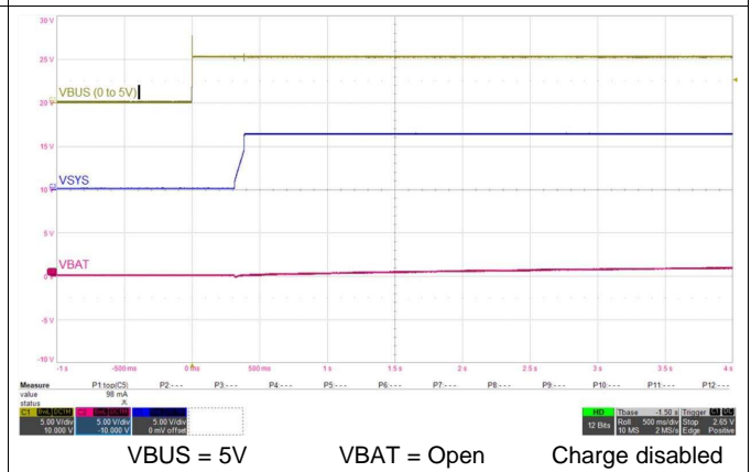
Figure 77. Adapter Plug-in with No Battery Charge Disabled
