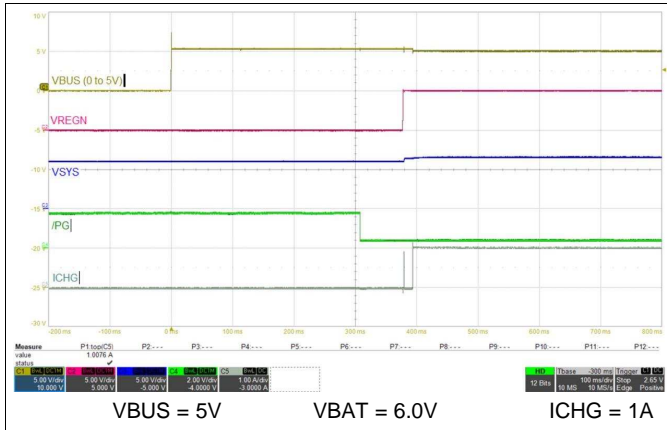
Figure 74. Adapter Power Up with Charge Enabled
