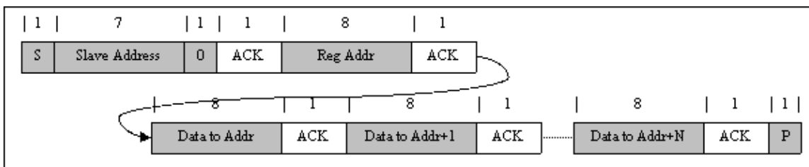
Figure 25. Multi-Write
