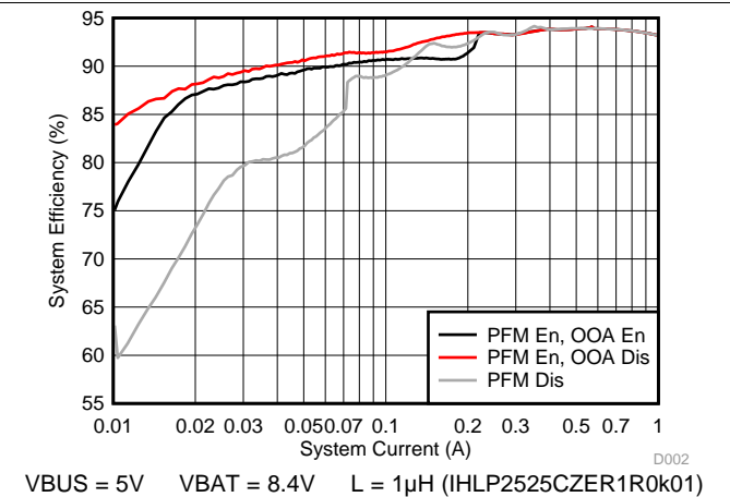
Figure 4. System Efficiency vs. System Current
