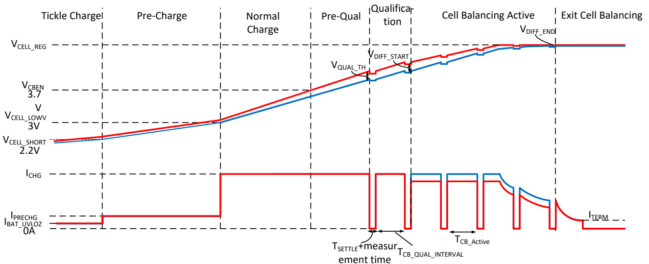
Figure 14. Cell Balancing Timing Diagram
