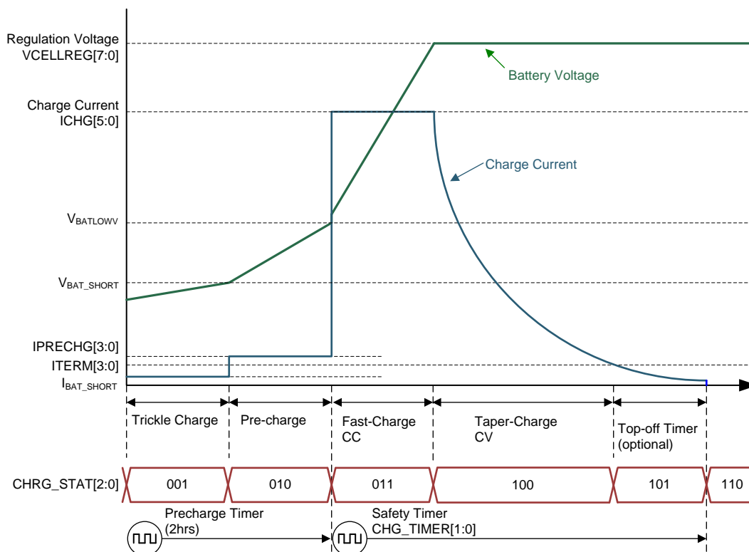
Figure 13. Battery Charging Profile
