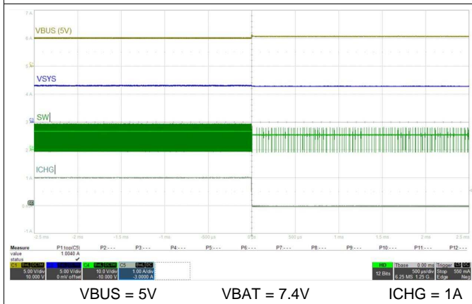
Figure 76. Charge Disabled
