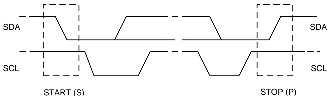
Figure 19. START and STOP conditions on the I2C bus
