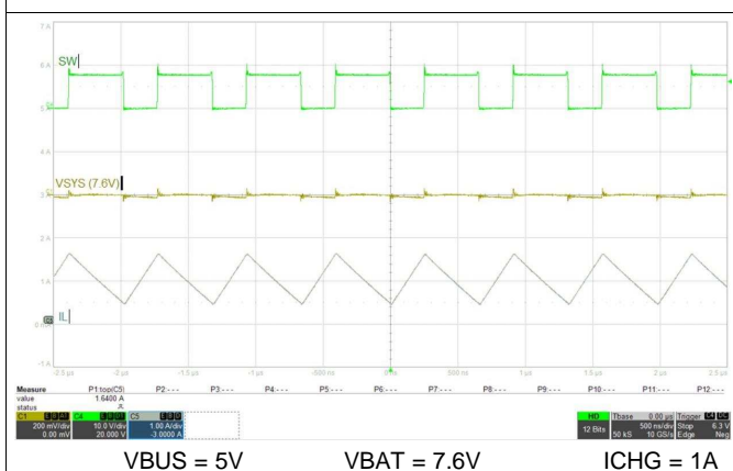
Figure 78. Boost Mode PWM Switching
