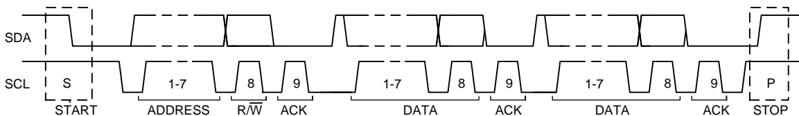
Figure 22. Complete Data Transfer on the I2C Bus
