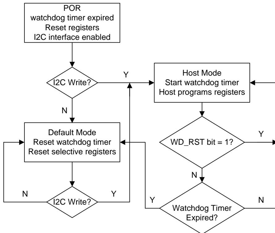
Figure 27. Watchdog Timer Flow Chart
