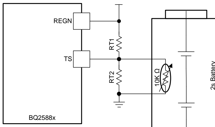
Figure 15. TS Resistor Network
