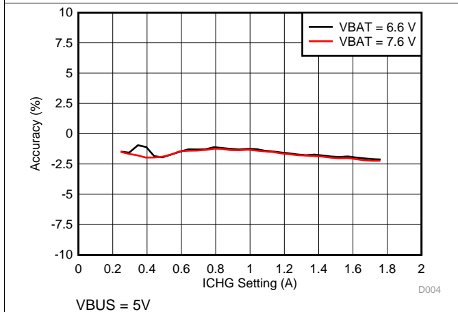
Figure 5. Charge Current Accuracy vs. ICHG Setting
