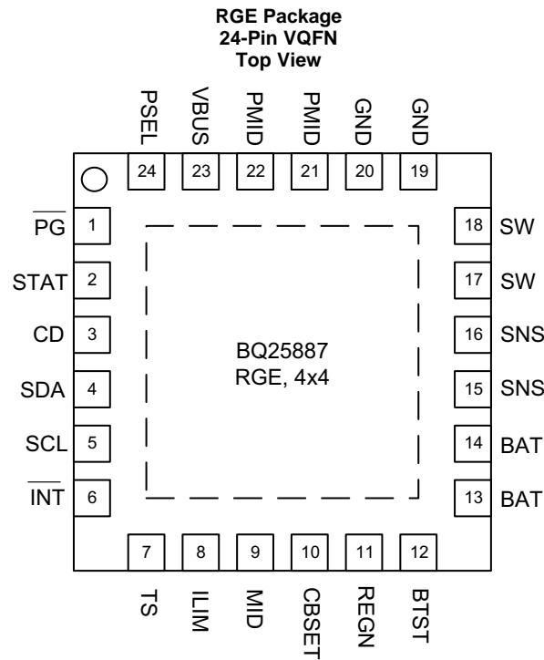
Pin Functions
