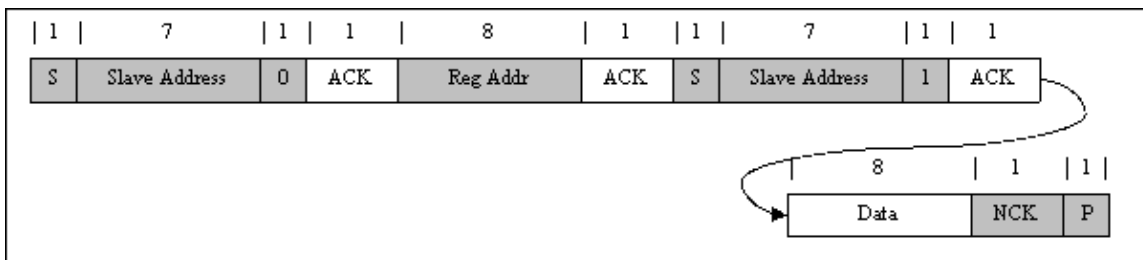
Figure 24. Single Read
