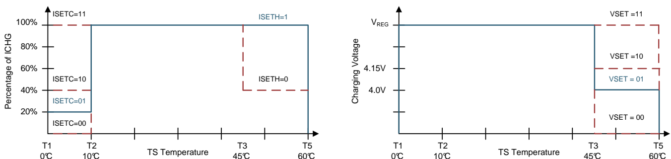
Figure 16. TS Charging Values
