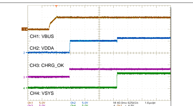
2-cell without battery
