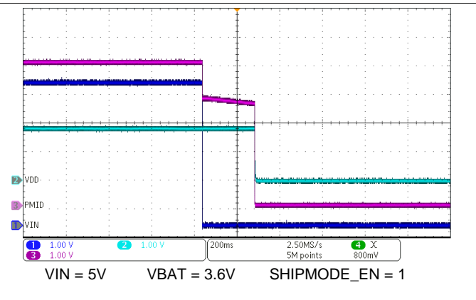
Figure 89. Ship Mode Entry on IN Supply Removal
