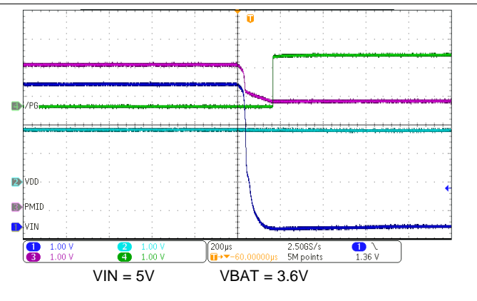
Figure 91. \overline{\text{PG}} Power Good Function - IN Supply Removal
