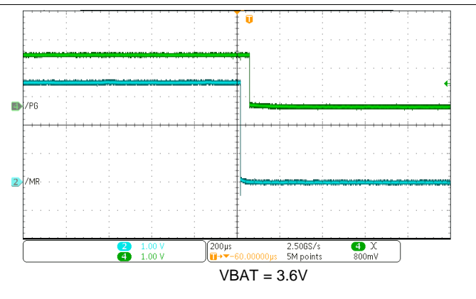
Figure 93. \overline{\text{PG}} \overline{\text{MR}} Level Shift Function - \overline{\text{MR}} Falling
