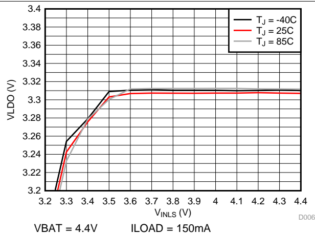
Figure 11. LDO Line Regulation (VLDO = 3.3V)
