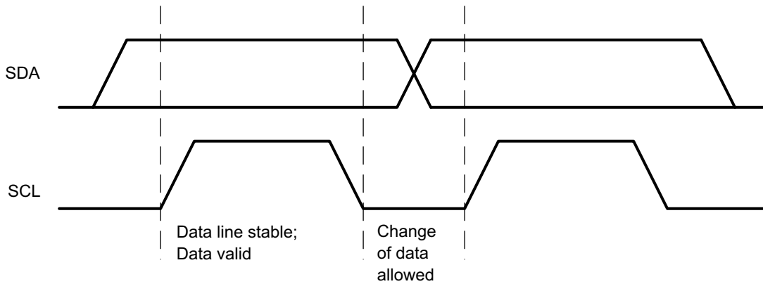
Figure 23. Bit Transfer on the I 2 C Bus
