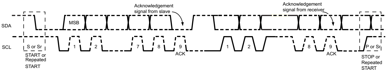
Figure 25. Data Transfer on the I 2 C Bus
