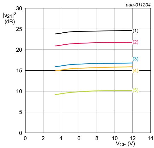
I_C = 25 mA; T_{amb} = 25 °C. (1) f = 300 MHz (2) f = 433 MHz (3) f = 800 MHz (4) f = 900 MHz (5) f = 1800 MHz
