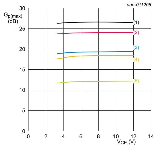
I_C = 25 mA; T_{amb} = 25 °C. If K > 1 then G_{p(max)} = maximum power gain. If K < 1 then G_{p(max)} = MSG. (1) f = 300 MHz (2) f = 433 MHz (3) f = 800 MHz (4) f = 900 MHz (5) f = 1800 MHz
