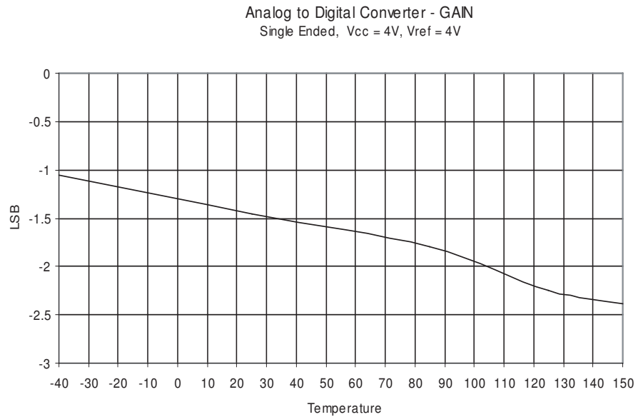
Figure 23. Analog to Digital Converter GAIN vs. Temperature, Single Ended
