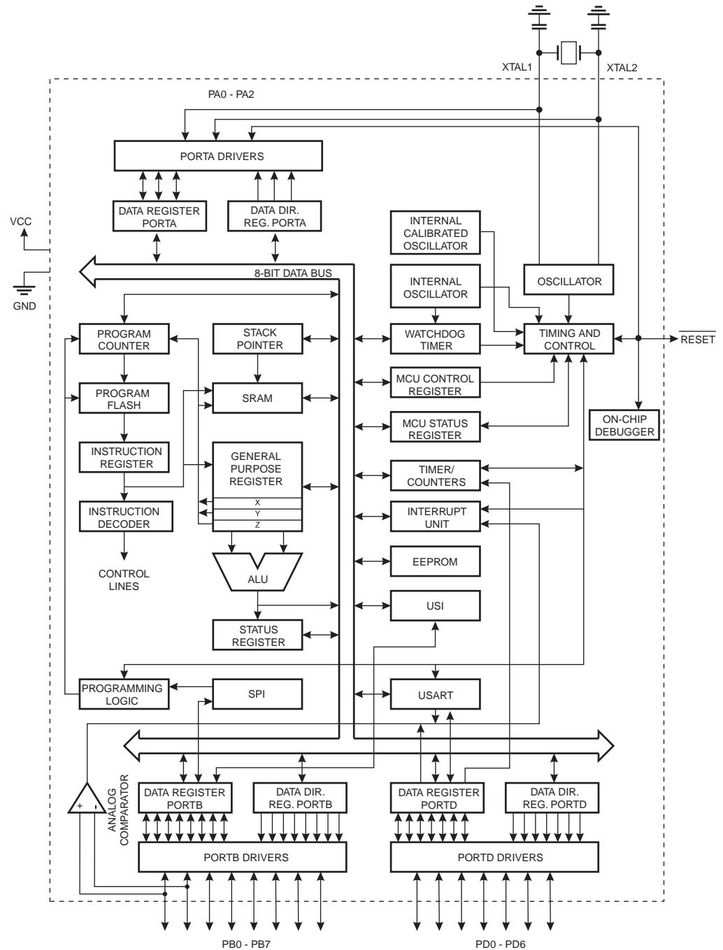
Figure 2-1. Block Diagram
