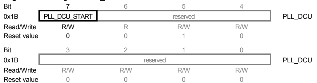
Figure 9-19. Register PLL_DCU.
