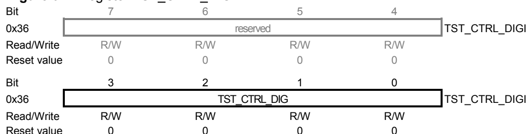
Figure 0-1. Register TST_CTRL_DIG.
