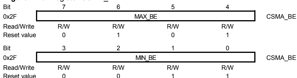
Figure 7-25. Register CSMA_BE.
