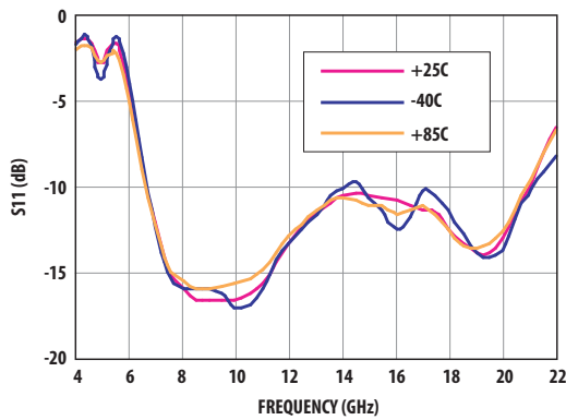
Figure 9. Input return loss over temperature.
