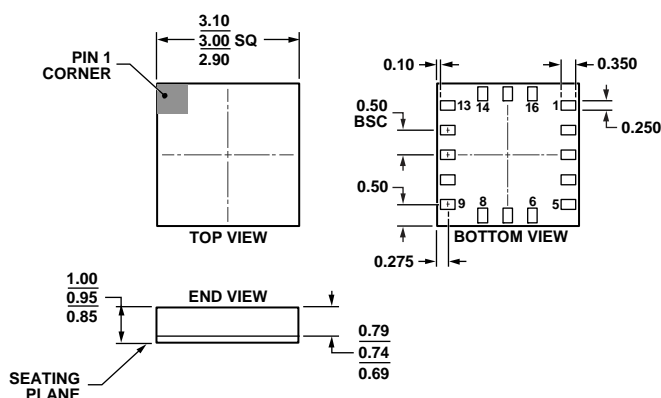
Figure 63. 16-Terminal Land Grid Array [LGA] (CC-16-3) Solder Terminations Finish Is Au over Ni Dimensions shown in millimeters
