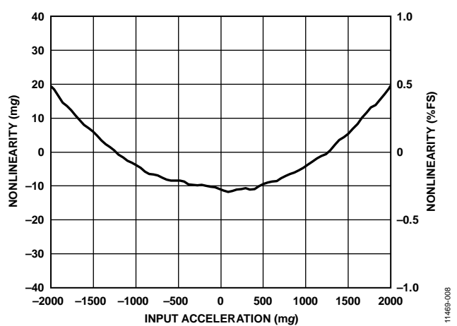
Figure 8. Z-Axis Nonlinearity, \pm 2 g Input Range
