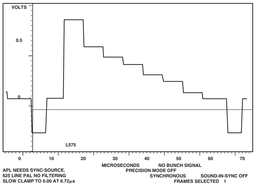
Figure 110. PAL Luma
