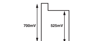
Figure 97. SD RGB Output Levels—RGB Sync Disabled
