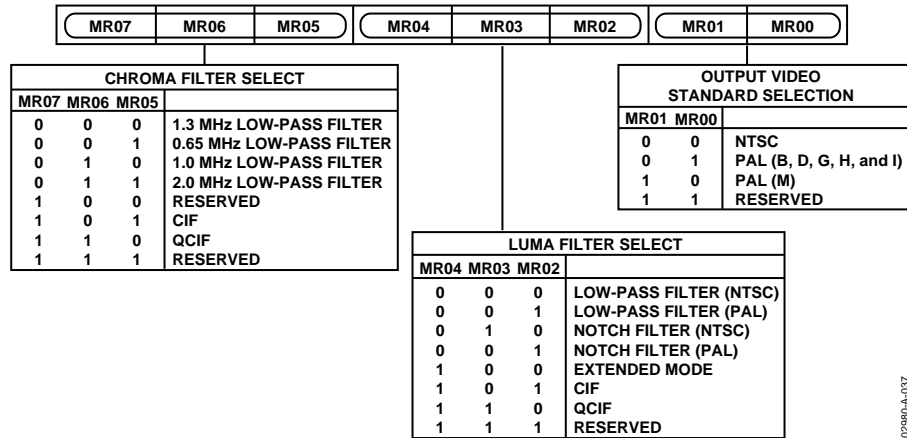
Figure 38. Mode Register 0
