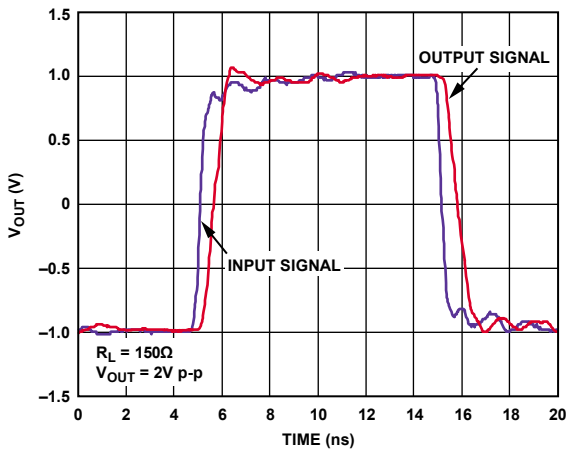
Figure 15. ADV3226 Large Signal Pulse Response
