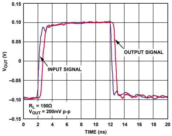
Figure 14. ADV3226 Small Signal Pulse Response
