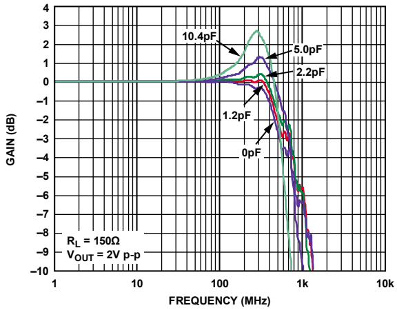
Figure 13. ADV3226 Large Signal Frequency Response with Capacitive Loads
