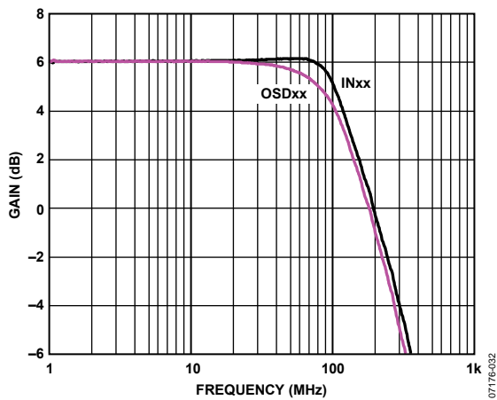
Figure 57. ADV3201 Large Signal Frequency Response, 2 V p-p
