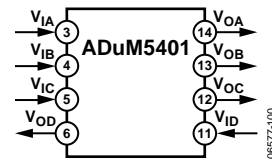
Figure 2. ADuM5401
