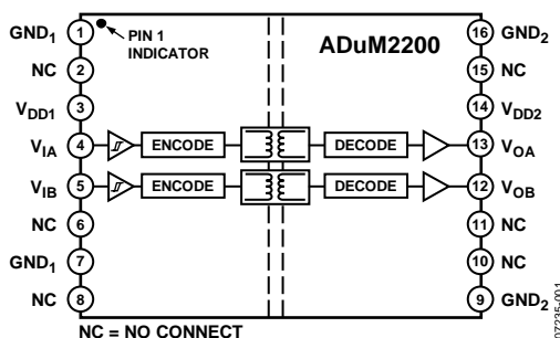
Figure 1. ADuM2200
